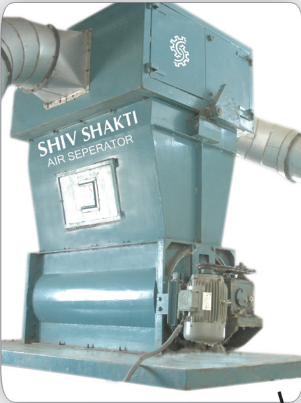
Air Separator
